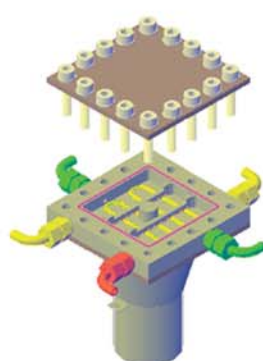
Temperature-controlled ultrasonic microreactor
